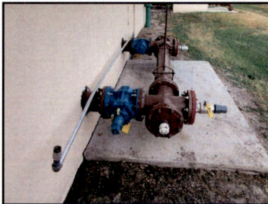
New Plug Valves Installed Between Digester #2 and Digester #3 Self-Leveling Pipes
